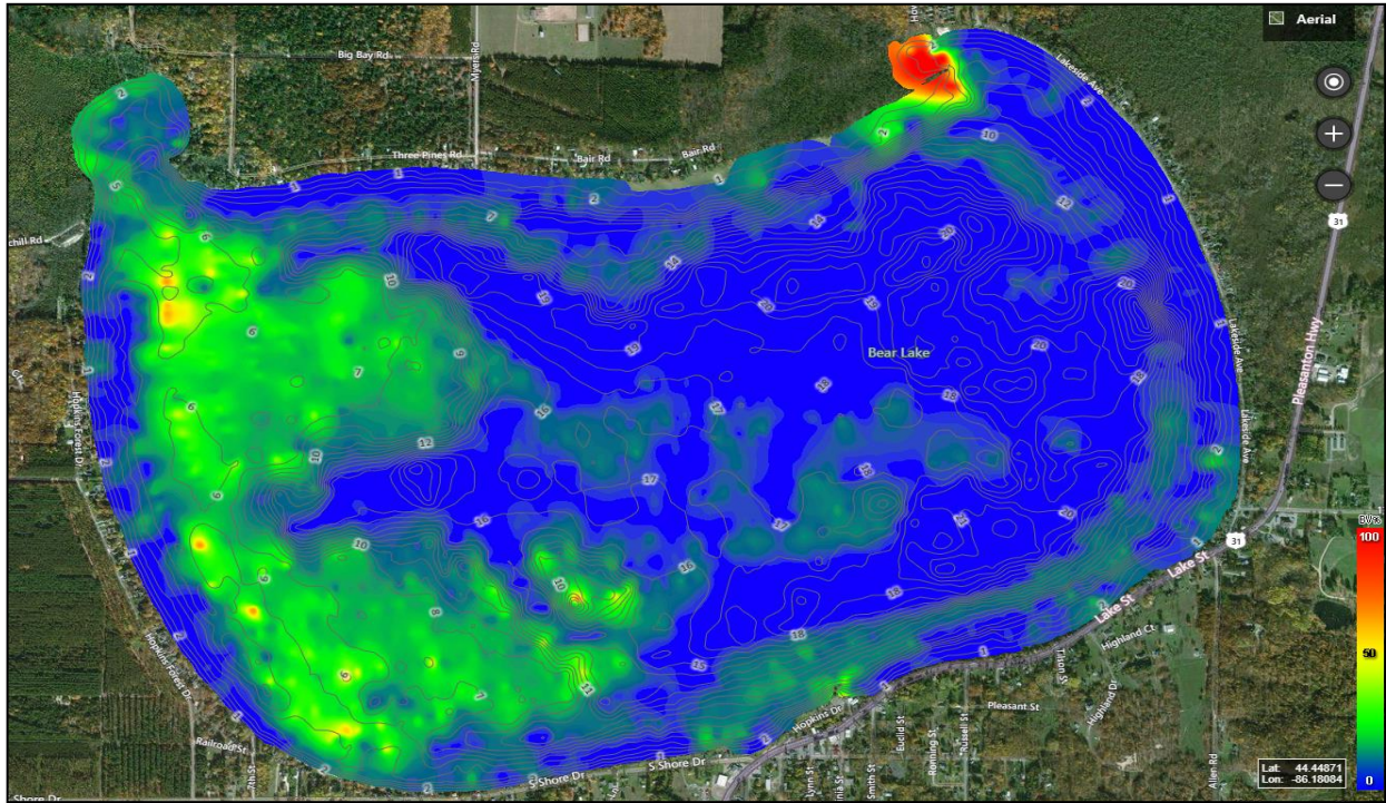
Figure 13. Aquatic Vegetation Biovolume in Bear Lake (August 19, 2020).
