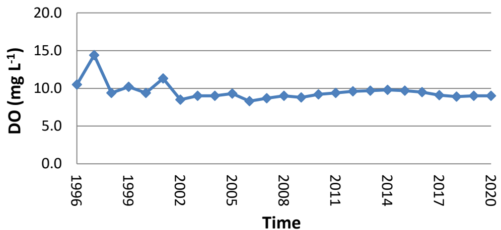
Figure 1. Temporal Trends in Mean DO among Bear Lake Deep Basins
