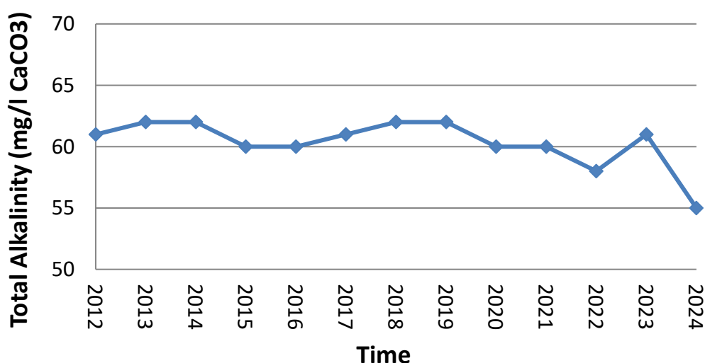
Figure 5: Temporal trends in mean total alkalinity within Bear Lake.
