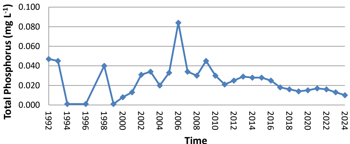
Figure 4. Temporal Trend in Mean TP among Bear Lake Deep Basins
