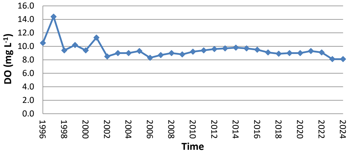
Figure 2: Temporal Trends in Mean Dissolved Oxygen in Bear Lake.
