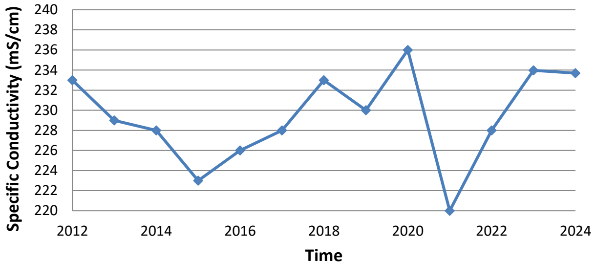
Figure 7. Temporal Trends in Mean Conductivity among Bear Lake Deep Basins
