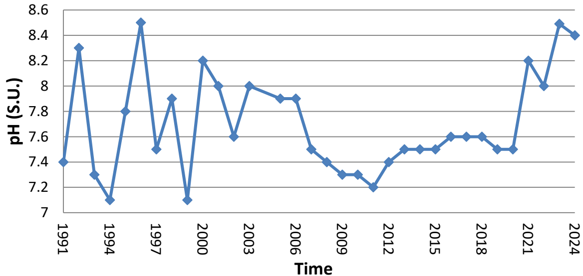
Figure 6: Temporal trends in mean pH within Bear Lake.
