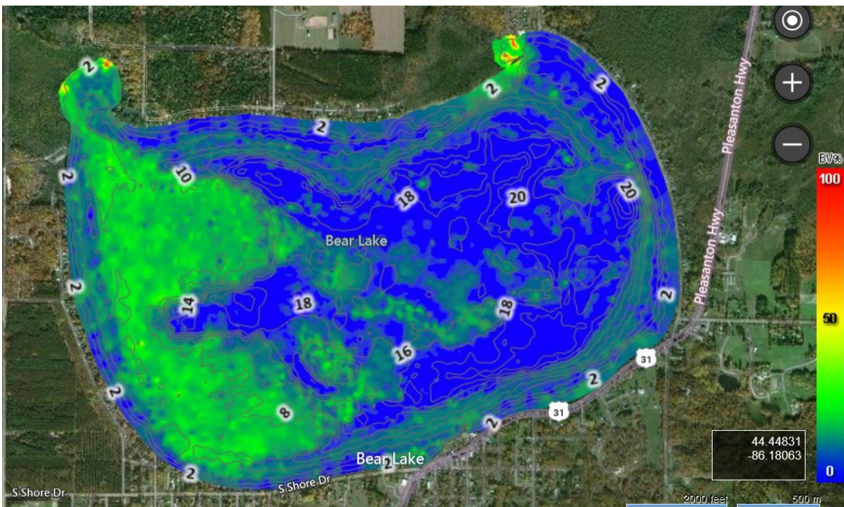
Figure 15: Bear Lake biovolume map from the August 1 st , 2024 survey. Most of the vegetation is located in the west basin of the lake in 3-12 feet depths. Blue = no vegetation, Red = Dense vegetation.
