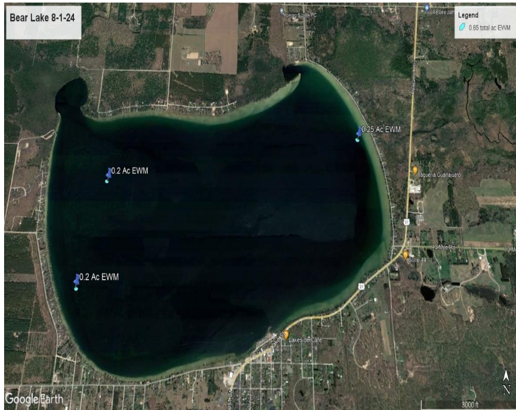
Figure 18. Distribution of EWM in Bear Lake (August 1, 2024).
